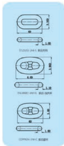
Mooring Chain-Studless Link Mooring Chain-Enlarged Link
