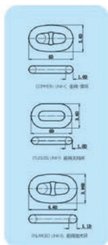
Anchor Chain-Enlarged Link
